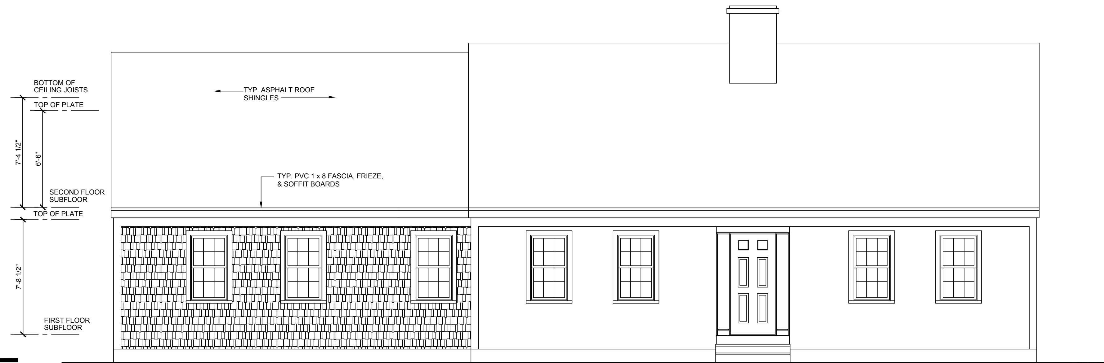
FRONT ELEVATION
