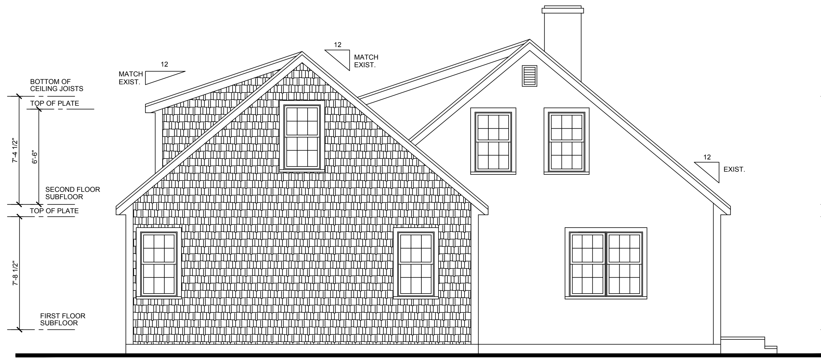
LEFT ELEVATION
