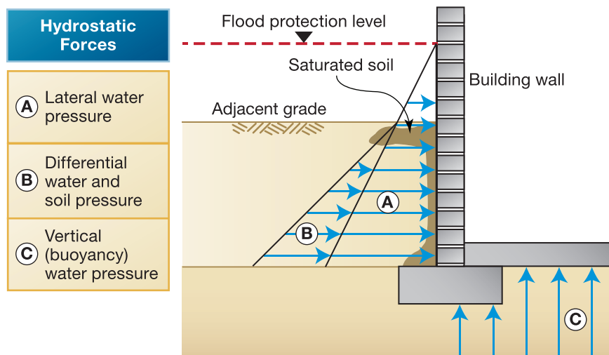
Figure 1-4. Hydrostatic forces.
